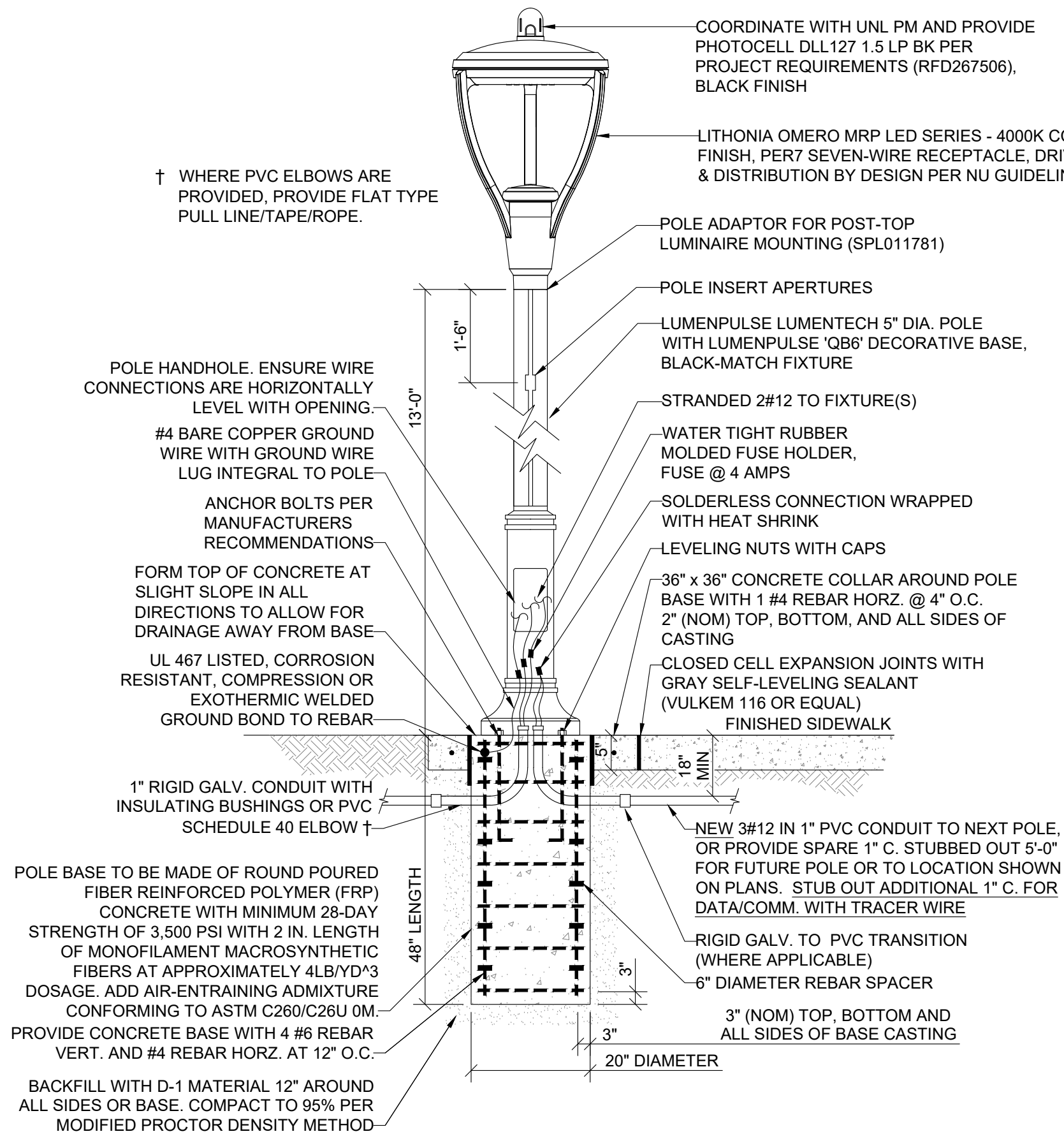
1 PEDESTRIAN POLE 'A' DETAIL E1.01 SCALE: NO SCALE
